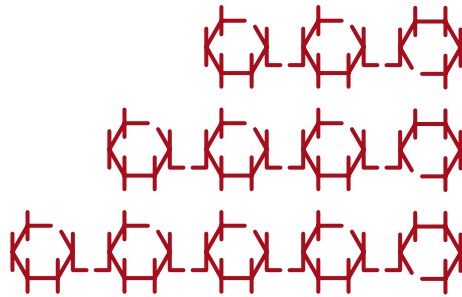
maltoligosyl glucoside > 50% (maltotriosyl glucoside)
